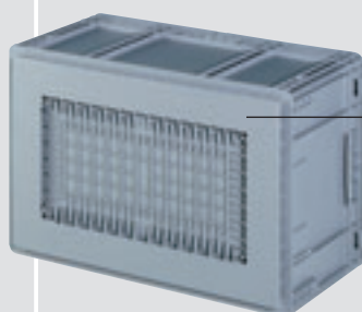
Standard base for and trouble-free and safe storage in the mini-load system (max. load 35 kg)
